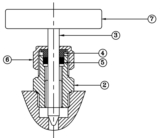
DETAILS OF BONNET-SPINDLE ASSEMBLY
